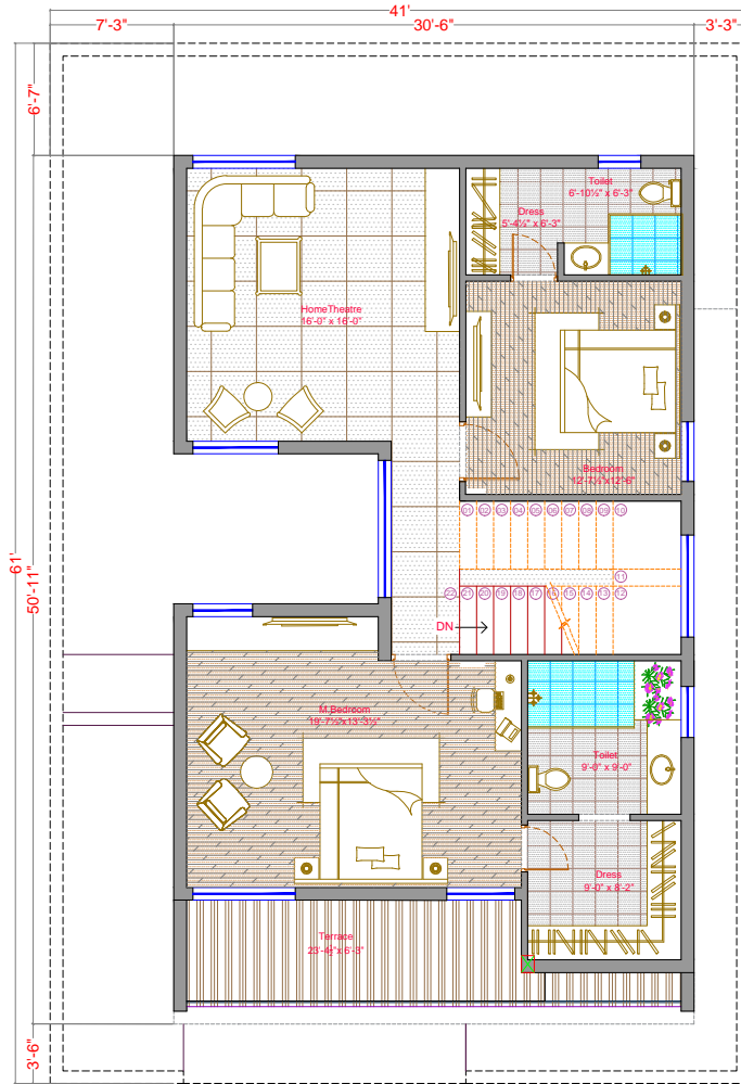
02 FIRST FLOOR PLAN 278 Sq yds west facing villa
