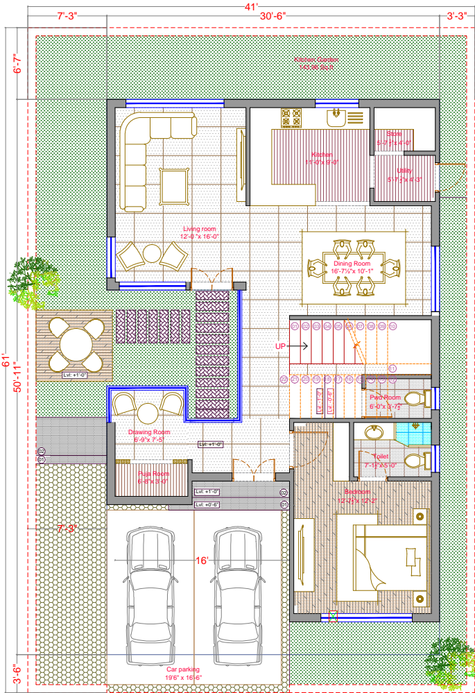
01 GROUND FLOOR PLAN 278 Sq yds west facing villa
